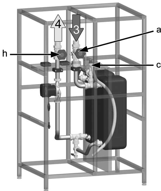
Secondary circuit
